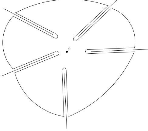
FIGURE 1. The cuts [\xi_j, \infty) and the contour \mathcal{G} .
